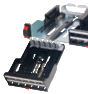
Copper system: simple extraction of connector blocks
